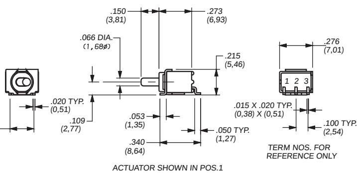
PC MOUNTING
