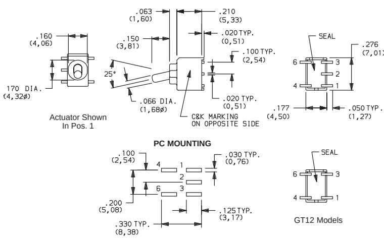
GT12-omit pad 2.
