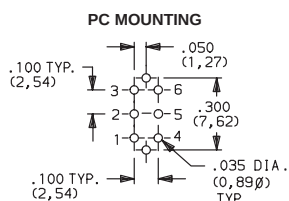
PC MOUNTING
