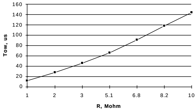
Figure 5. Bias resistance vs pulse width. R in MΩ.
