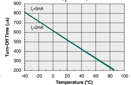
Typical Turn-Off vs. Temperature ( I_L=70\text{mA} )
