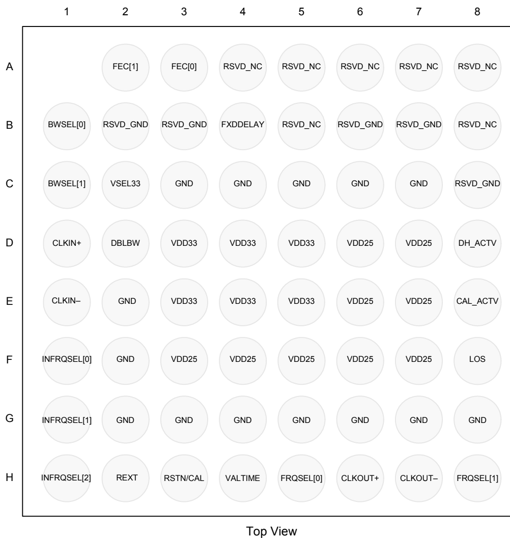
Figure 12. Si5320 Pin Configuration (Transparent Top View)
