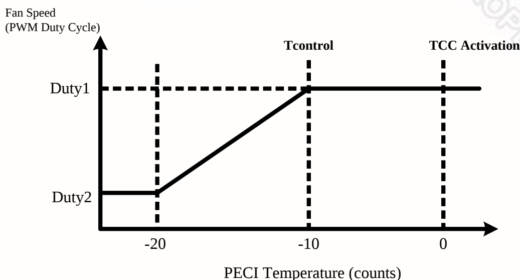
Figure 8-8 PECI Temperature
