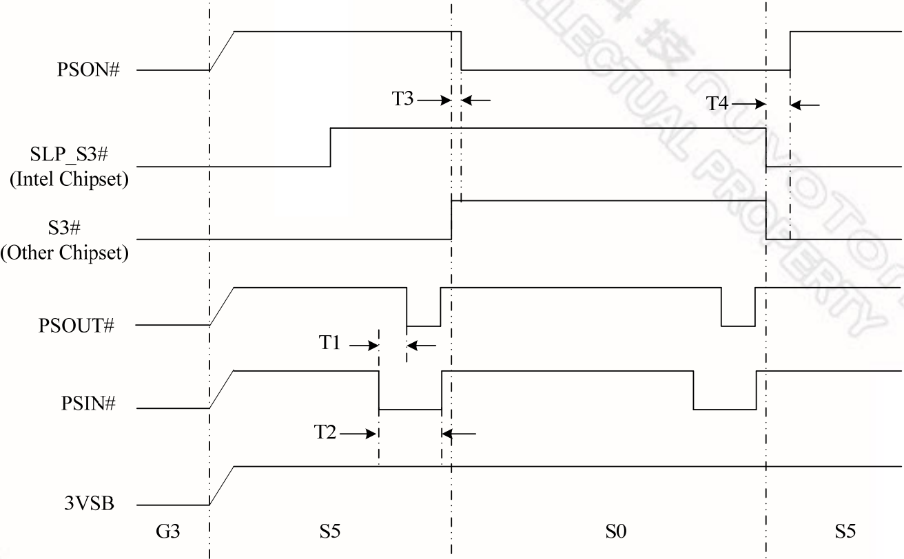
Figure 14-2 Power Sequence from S5 to S0, then Back to S5
