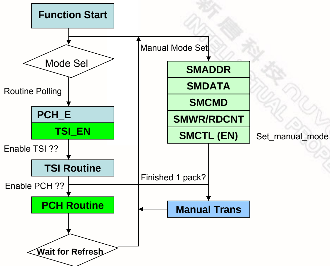
Figure 18-5 Programming Flow
