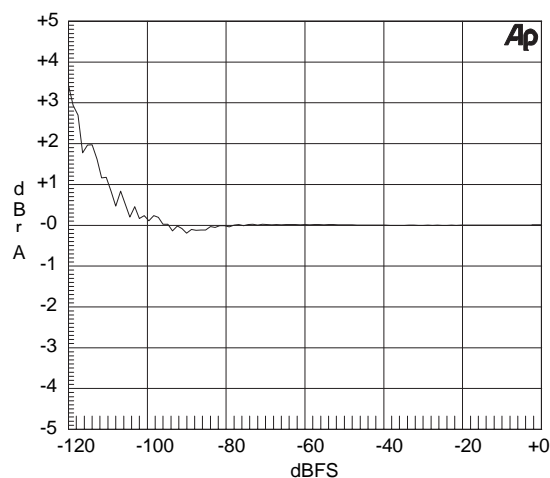
Figure 19. Fade-to-Noise Linearity
