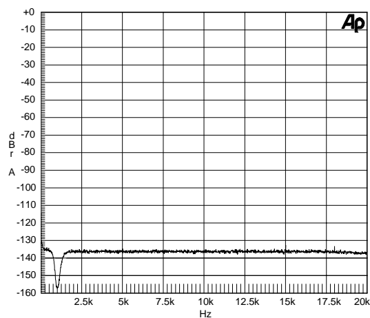
Figure 17. -20 dBFS FFT
