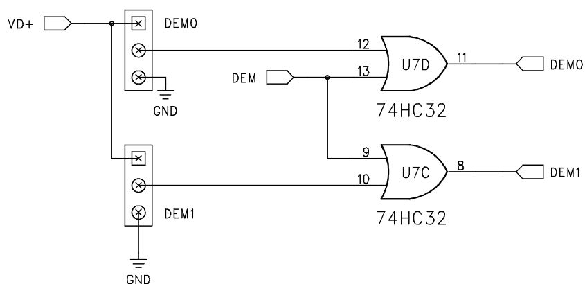
Figure 3. De-emphasis Circuitry
