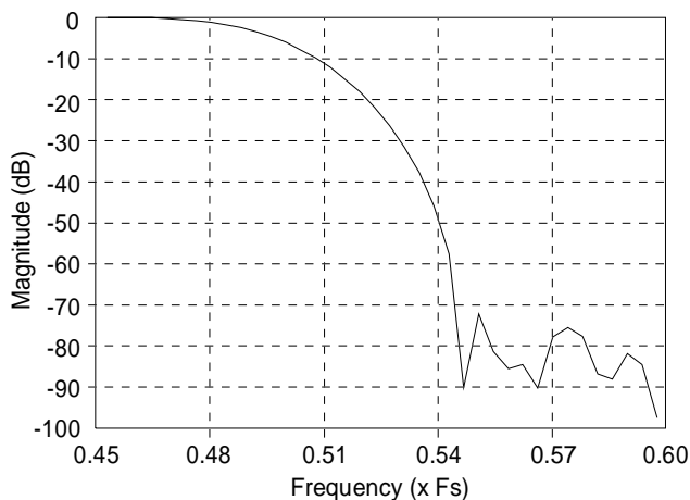
Figure 10. CS4329 Combined Digital and Analog Filter
