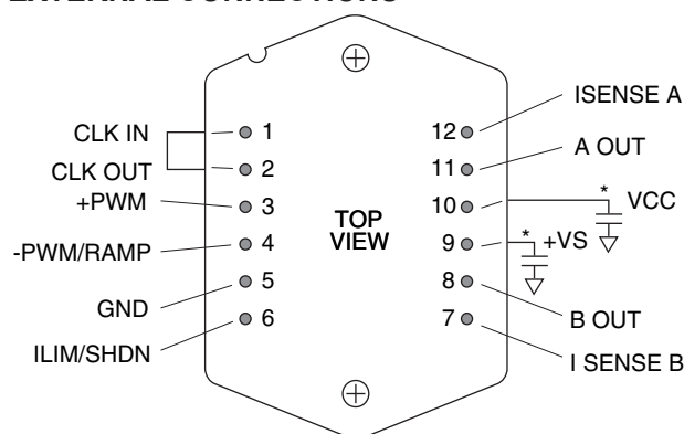
12-PIN POWER DIP PACKAGE STYLE CR
