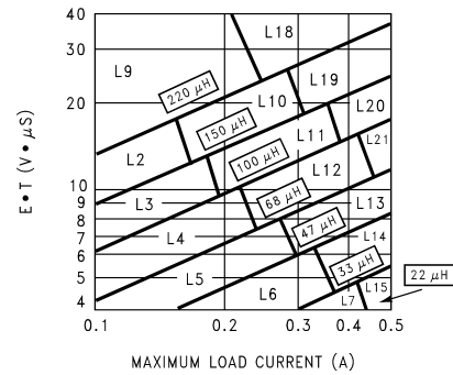
Figure 7-13. LM2674, Adjustable Version
