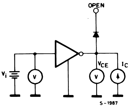
Figure 8. Input voltage
