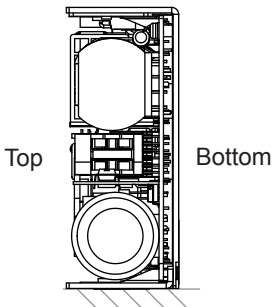
Fig. 4: Mounting on the right side
