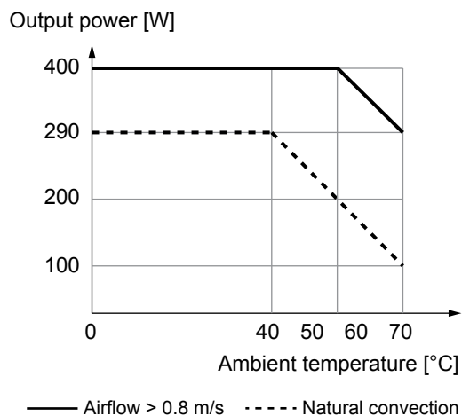
Fig. 7: Output power versus ambient temperature 12 V
