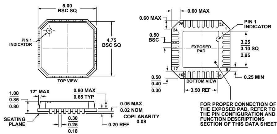
Figure 91. 32-Lead Lead Frame Chip Scale Package [LFCSP_VQ] 5 mm x 5 mm, Very Thin Quad (CP-32-2) Dimensions shown in millimeters
