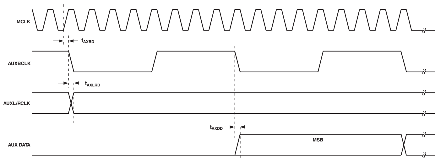
Figure 5. Auxiliary Interface Timing
