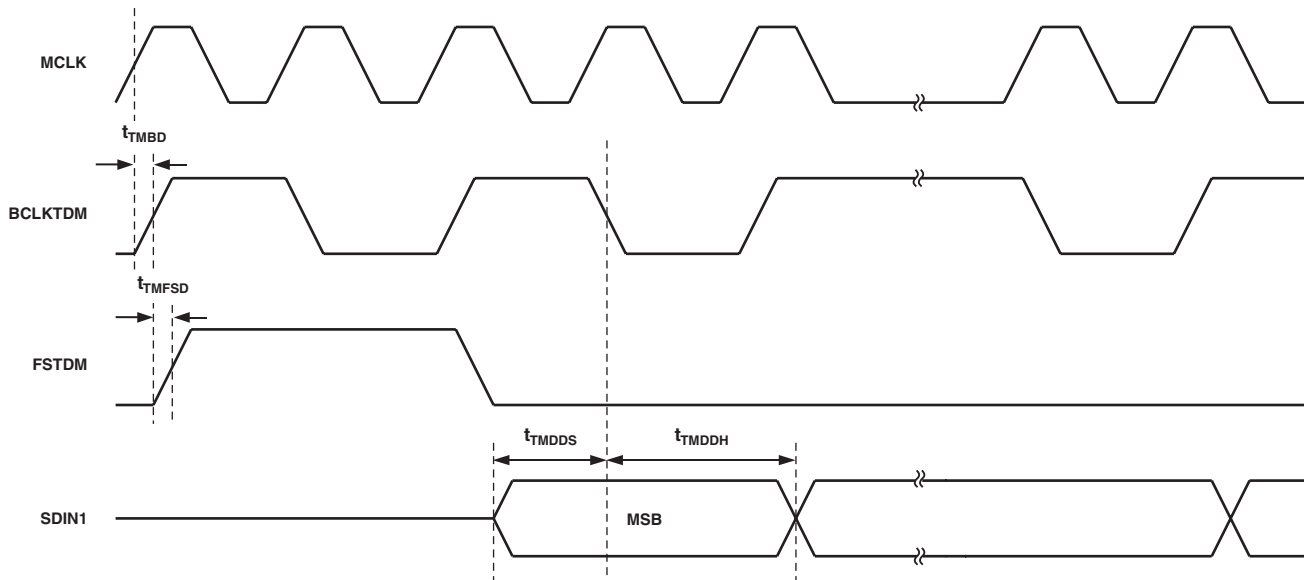
Figure 4. TDM Master Mode Timing
