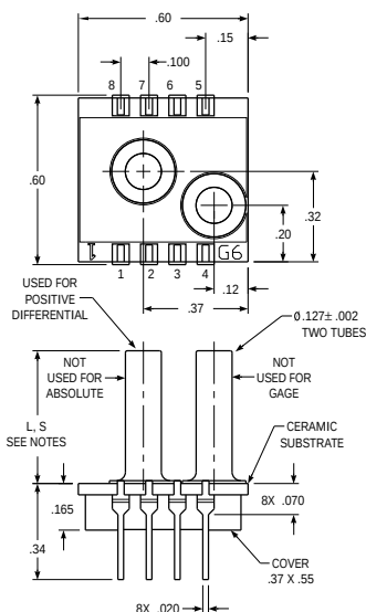
Package Diagram
