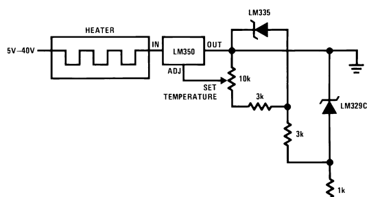
Simple Temperature Control
