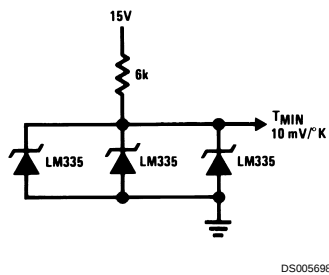
Minimum Temperature Sensing
