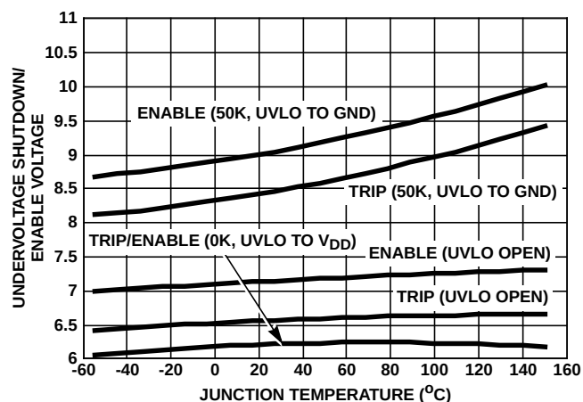
FIGURE 16. UNDERVOLTAGE THRESHOLD
