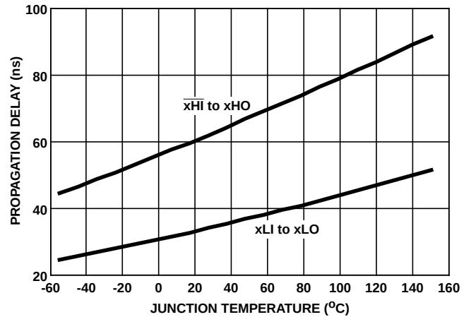
FIGURE 12. PROPAGATION DELAY
