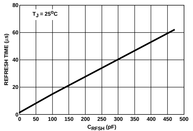
FIGURE 14. REFRESH TIME
