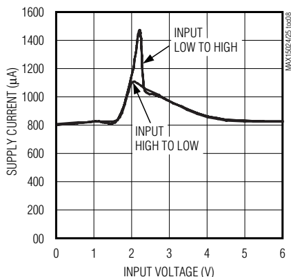
SUPPLY CURRENT vs. LOGIC IN
