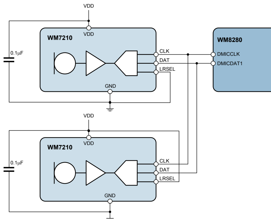
Figure 2 Stereo WM7210 Digital Microphone Connection to WM8280
