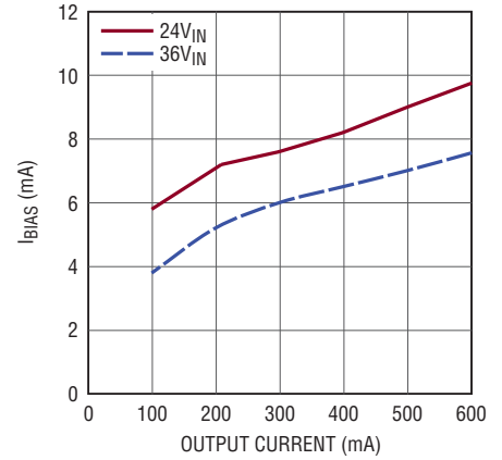
I_{\text{BIAS}} vs Output Current, 18V_{\text{OUT}} , BIAS = 5V
