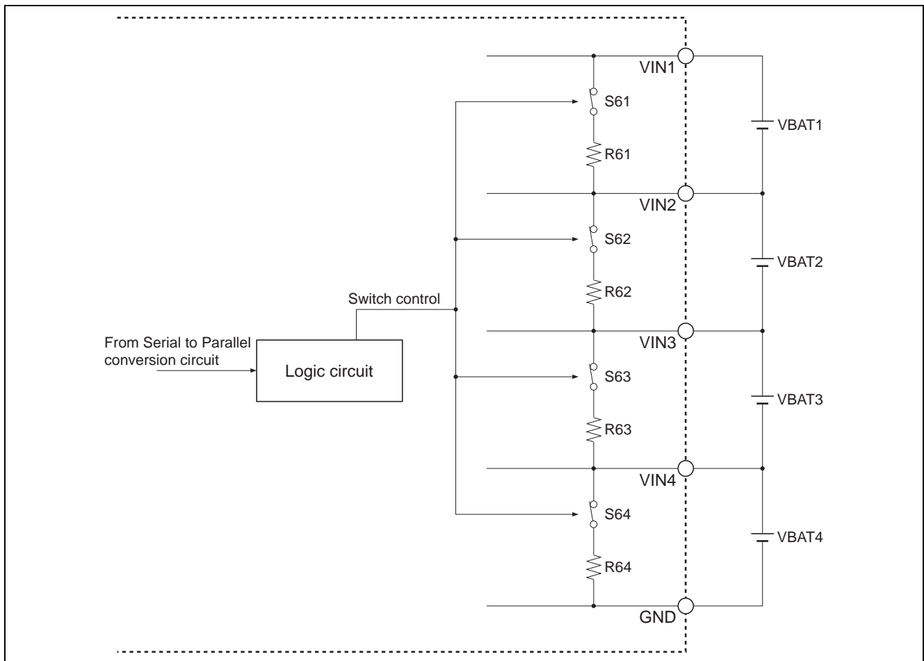
Figure 7 Conditioning Circuit
