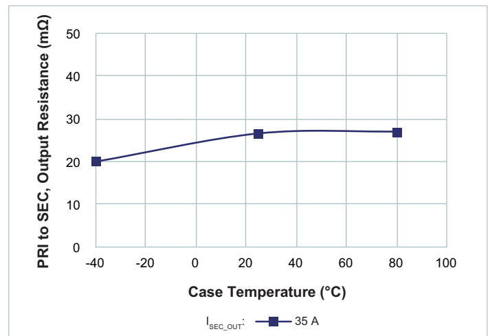
Figure 9 — R_{SEC} vs. temperature; Nominal V_{PRI\_DC} I_{SEC\_DC} = 24\text{ A} at T_{CASE} = 80^\circ\text{C}
