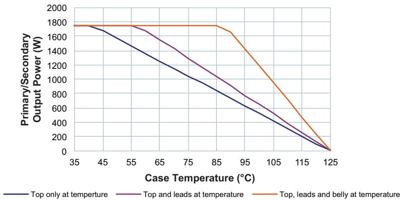
Figure 1 — Specified thermal operating area
