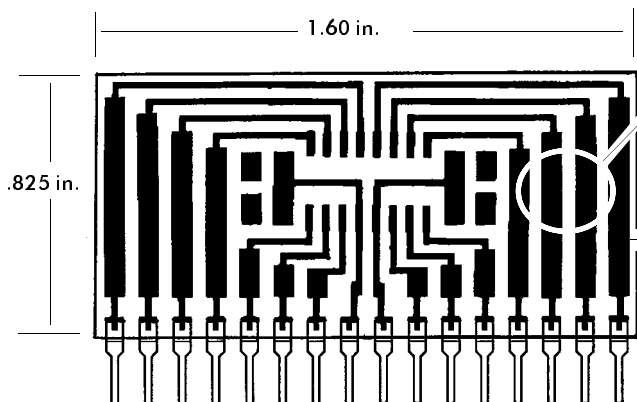
SINGLE-IN-LINE (SIP) PINS ON .100 in. CENTERS
