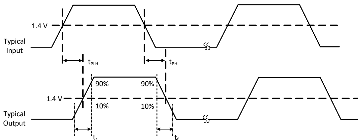
Figure 12. Propagation Delay Timing
