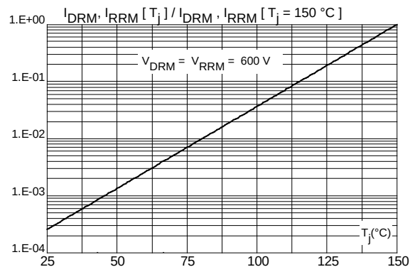
Figure 11: Relative variation of leakage current versus junction temperature ( t_p < 10 ms)
