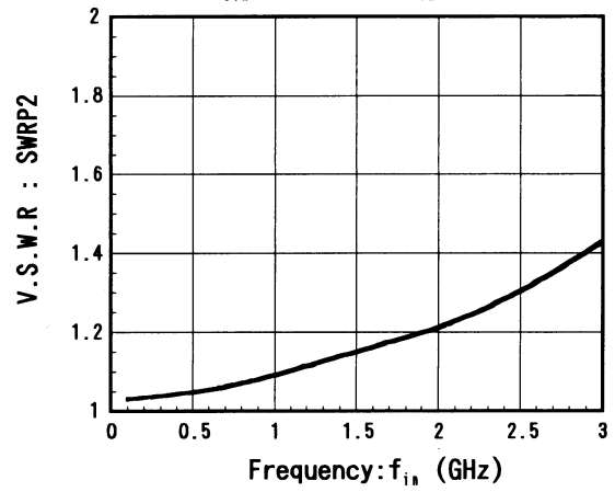
P2-PC(ON) V.S.W.R vs. Frequency
