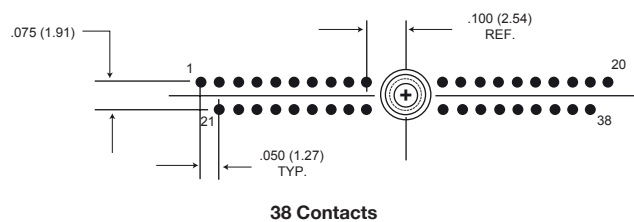
38 Contacts
