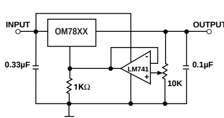
Adjustable Output Regulator, 7 To 30 Volts
