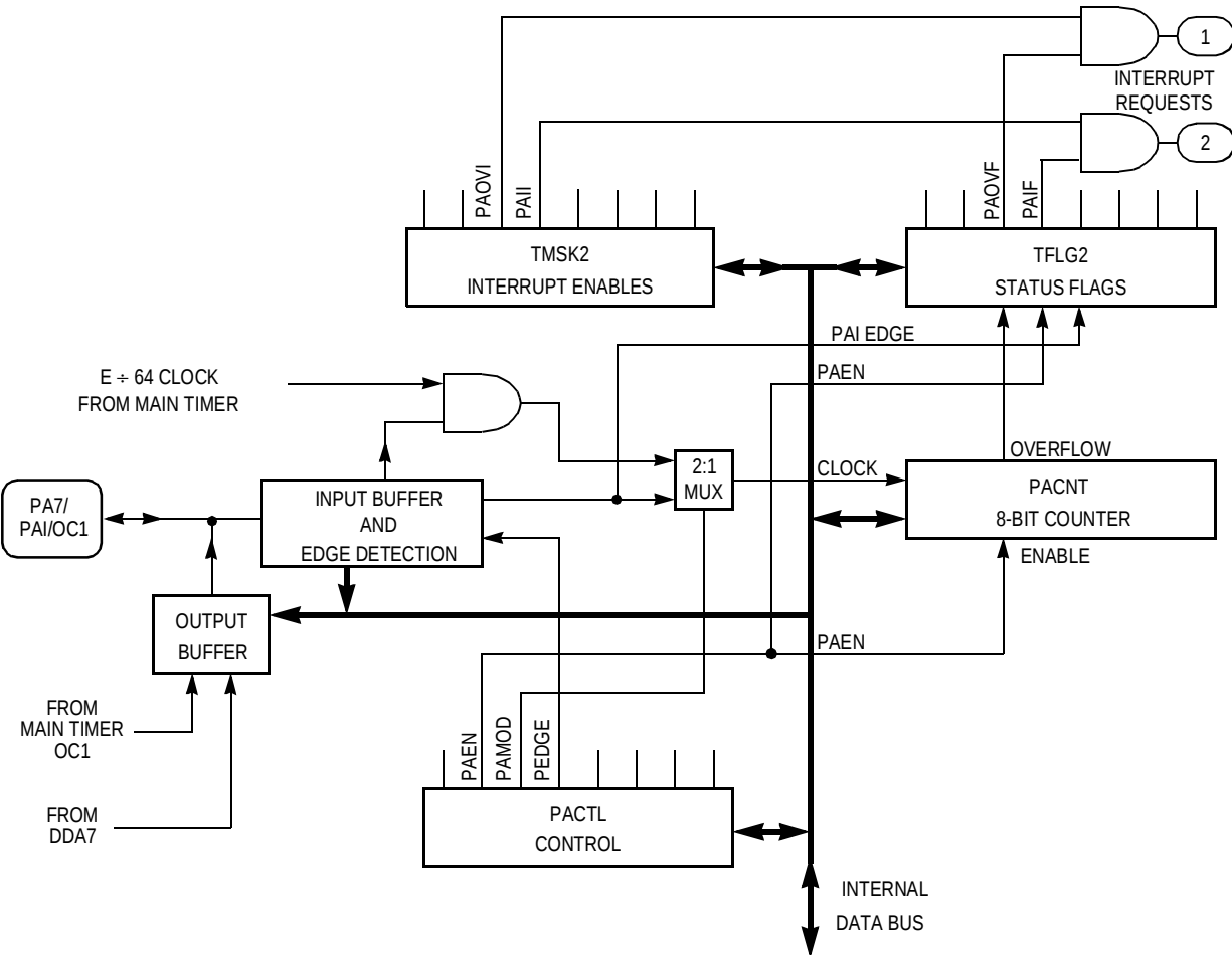
Figure 9-21. Pulse Accumulator
