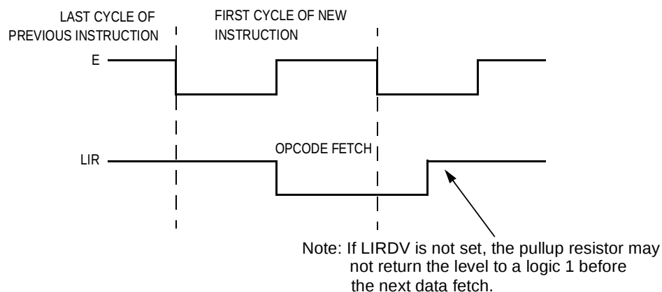
Figure 2-8. \overline{LIR} Timing
