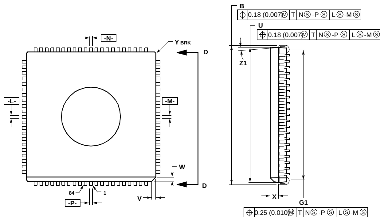
DETAIL D-D
