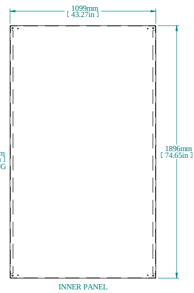
INNER PANEL
