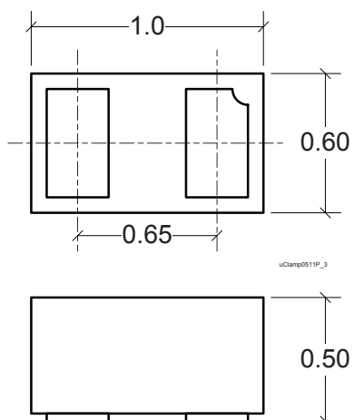
Nominal Dimensions (mm)
