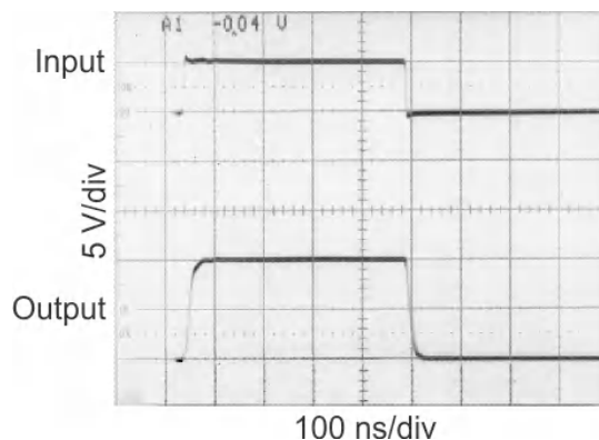
Figure 6-9. Isolation Resistor Used to Drive Capacitive Load
