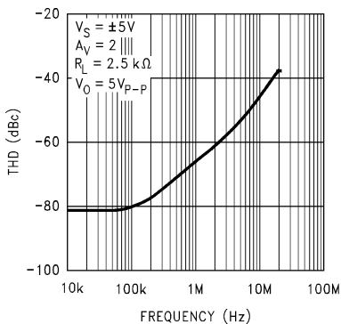
Figure 5-86. Total Harmonic Distortion vs Frequency
