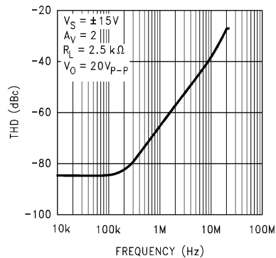
Figure 5-85. Total Harmonic Distortion vs Frequency
