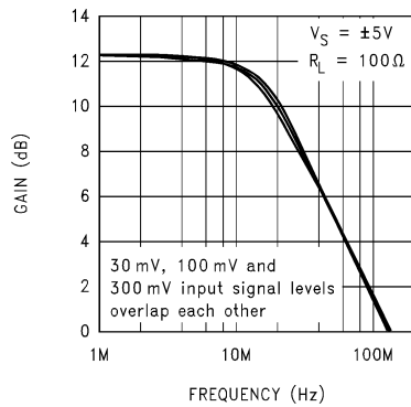
Figure 5-84. Closed-Loop Frequency Response vs Input Signal Level
