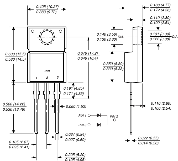
ITO-220AB (SBLF25LxxCT)
