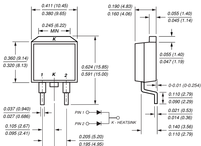
TO-263AB (SBLB25LxxCT)
