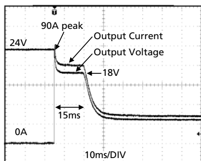
Fig. 23-3 90A Peak load, typ.
