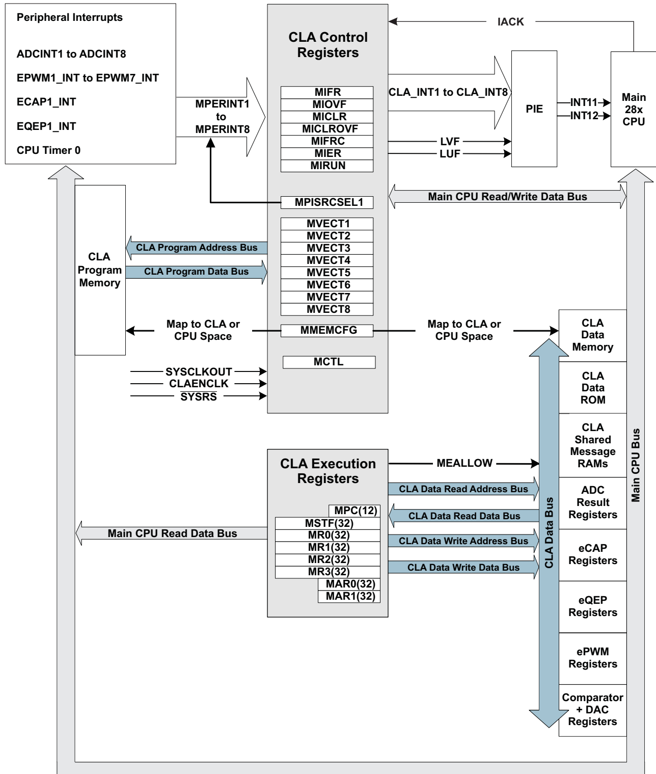
Figure 6-2. CLA Block Diagram
