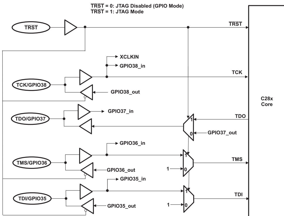
Figure 6-29. JTAG/GPIO Multiplexing
