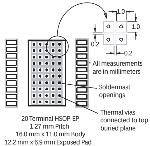
Figure 25. Thermal Land Pattern for Direct Thermal Attachment According to JESD51-5
