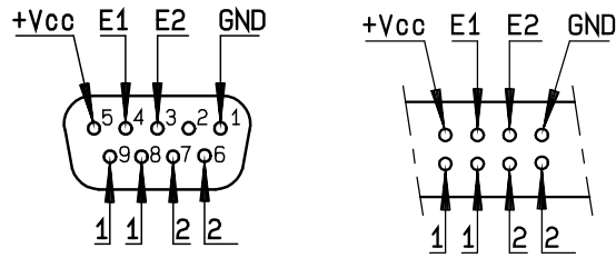
D-Sub connector
