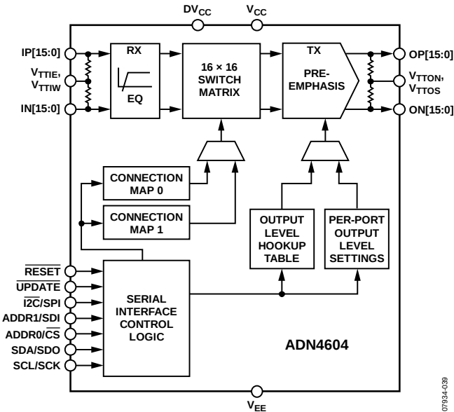
Figure 39. Block Diagram
