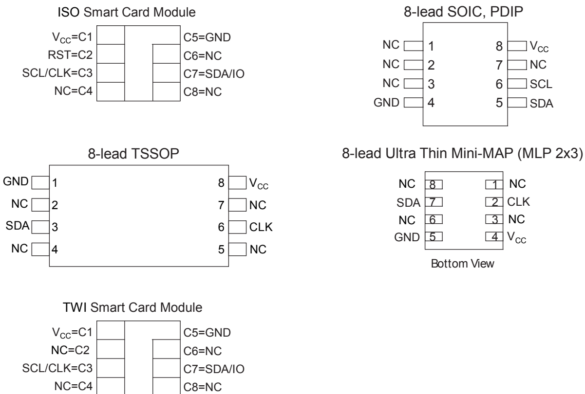
Figure 1. Pin Configuration
