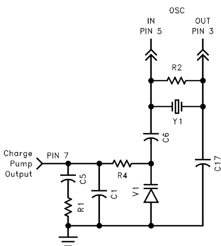
FIGURE 14. XTAL
