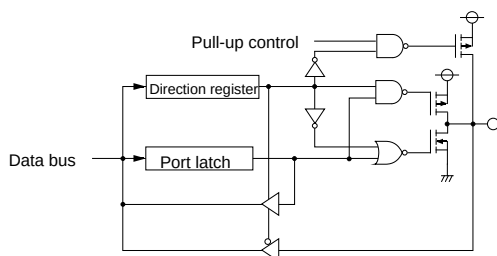
(8) Ports P30–P35
