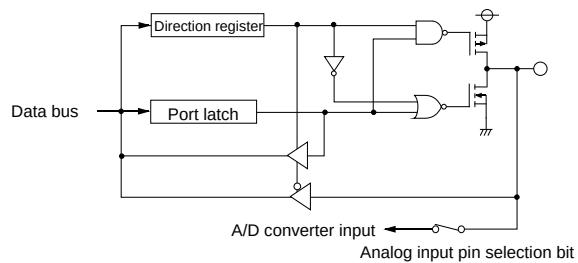
(7) Ports P20–P27
