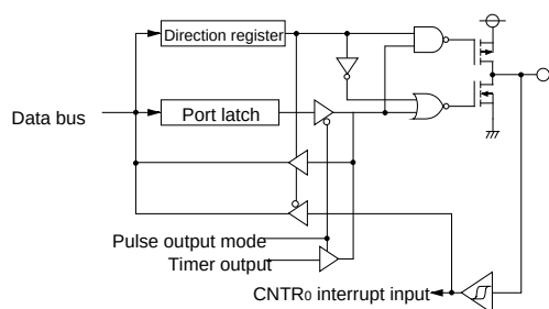
(6) Ports P14
