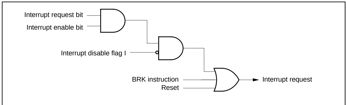
Fig. 16 Interrupt control
