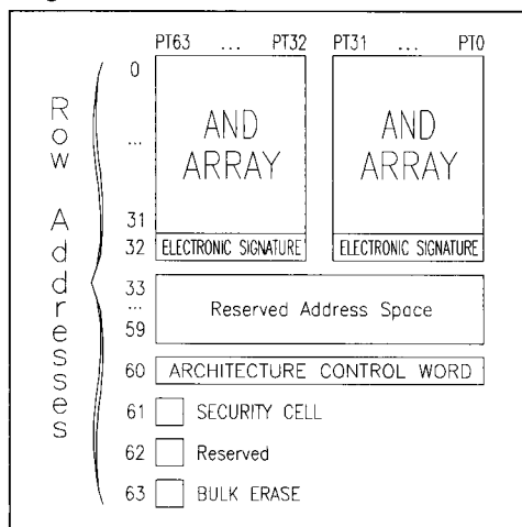
GAL16V8AS Row Addresses Map Block Diagram
