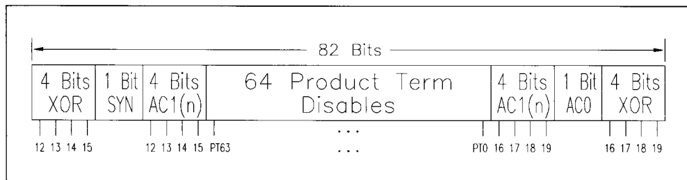
GAL16V8AS Architecture Control Word Diagram
