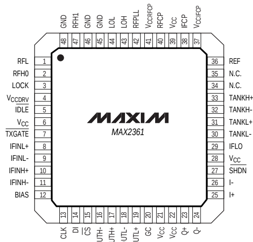
(T) QFN-EP
