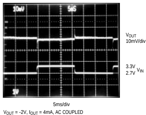
LINE-TRANSIENT RESPONSE
