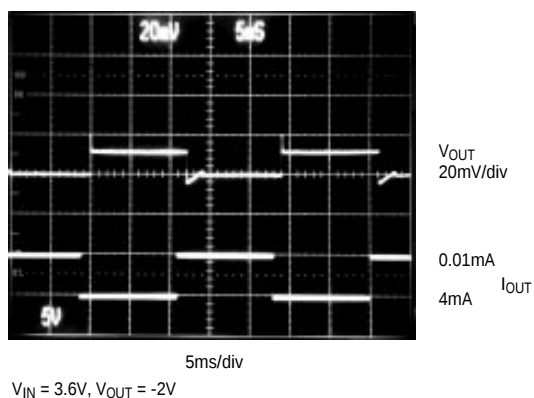
LOAD-TRANSIENT RESPONSE
