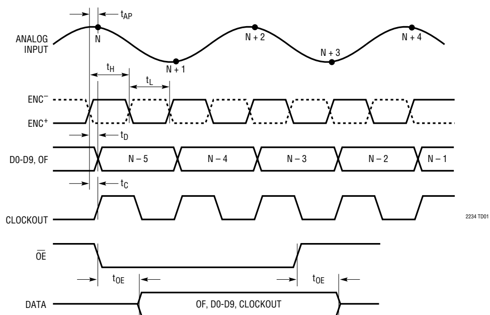
Timing Diagram
