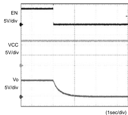
Fig.4 Waveform at output OFF \text{Co}=1\mu\text{F}
