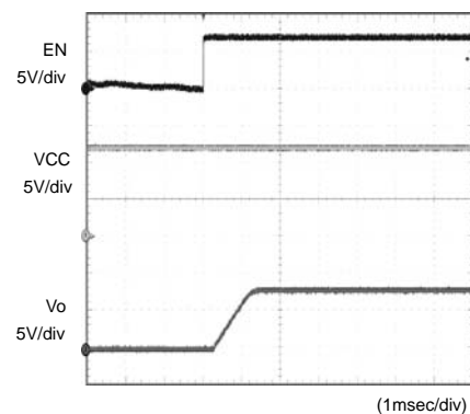
Fig.5 Input sequence 1 \text{Co}=1\mu\text{F}
