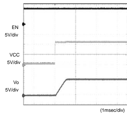
Fig.6 Input sequence 2 \text{Co}=1\mu\text{F}
