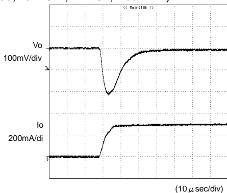
Fig.2 Transient Response (0→50mA) \text{Co}=1\mu\text{F}
