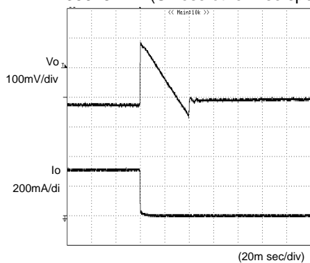
Fig.1 Transient Response (50→0mA) \text{Co}=1\mu\text{F}
