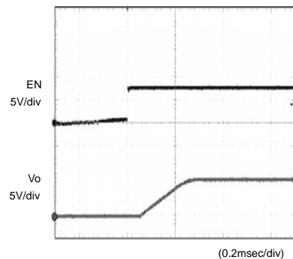
Fig.3 Waveform at output start \text{Co}=1\mu\text{F}
