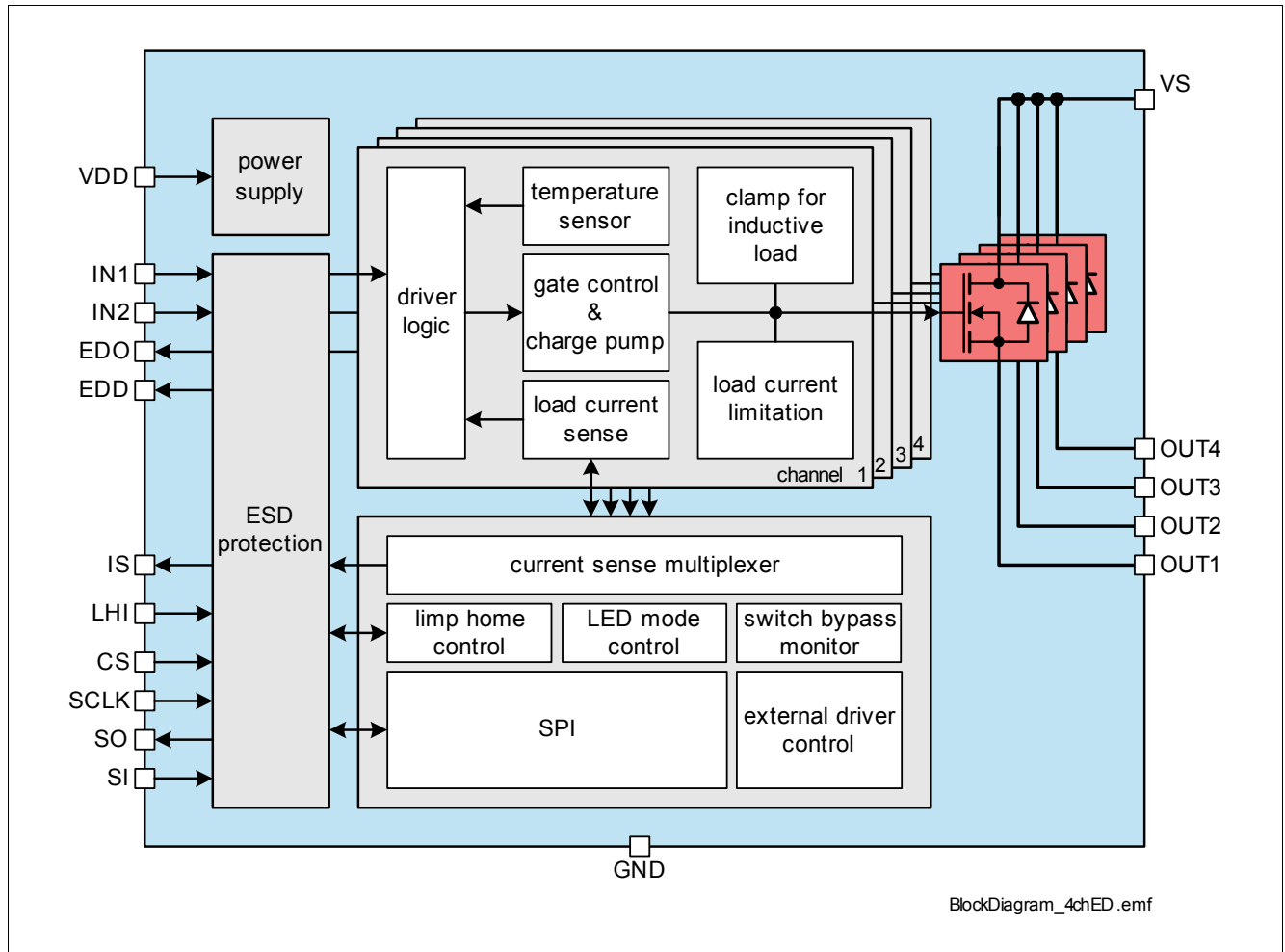
Figure 1 Block Diagram BTS54040-LBF
