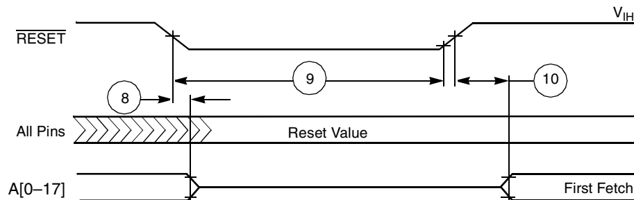
Figure 2-3. Reset Timing
