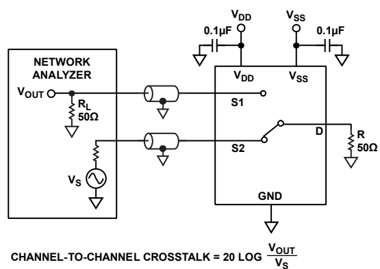
Figure 30. Channel-to-Channel Crosstalk
