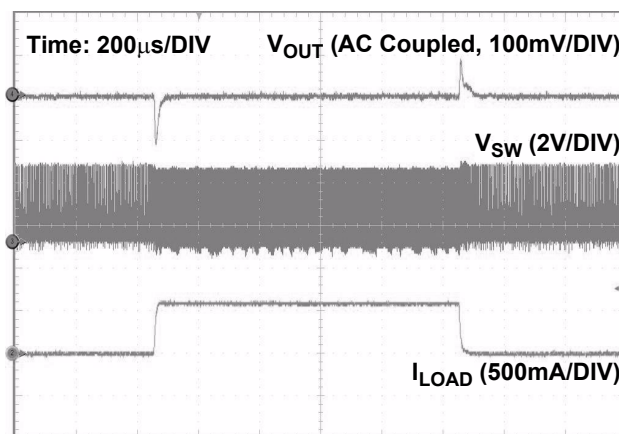
Figure 12. Load Transient in Z-mode V_{IN} = 3.6V , I_{LOAD} = 10mA to 600mA
