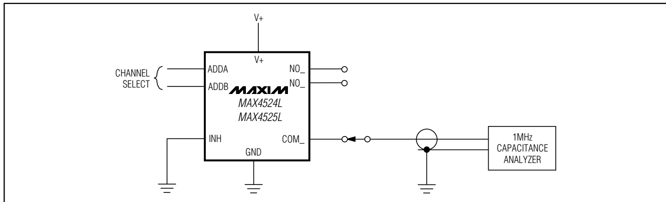
Figure 5. NO/COM Capacitance
