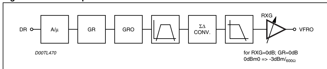
Figure 5. Receive path
